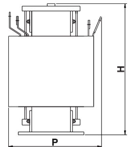
Fig. 1: Three phase transformer with exits on screw clamps (up to 80 kVA rated power)
